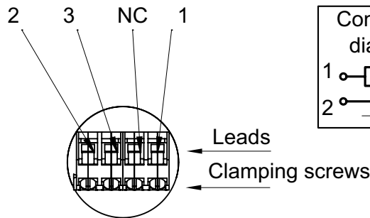
Option KA (on request) pin Assignment (rear view)
